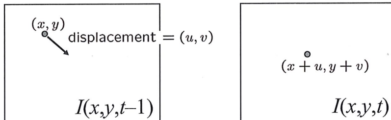
Figure 3. I(x, y, t) denotes the brightness of a pixel at position (x, y) at time instant t .
